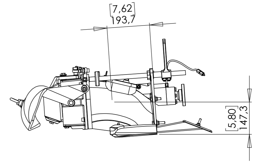
COG without adapter SCALE 1 : 10
